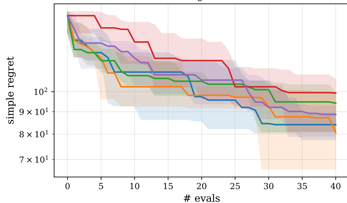
Rastrigin-10D
