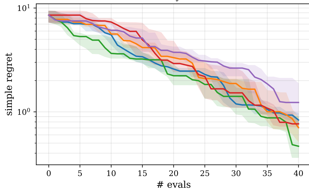
Rastrigin-10D
