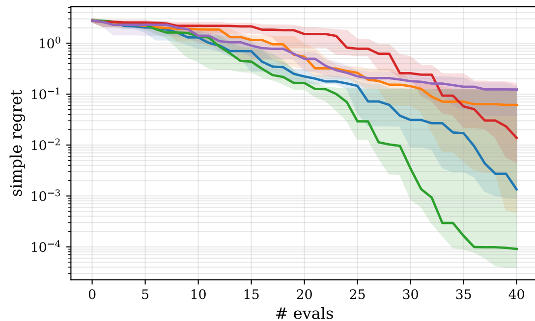
Ackley-20D
