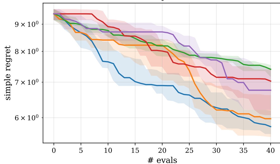
Ackley-20D
